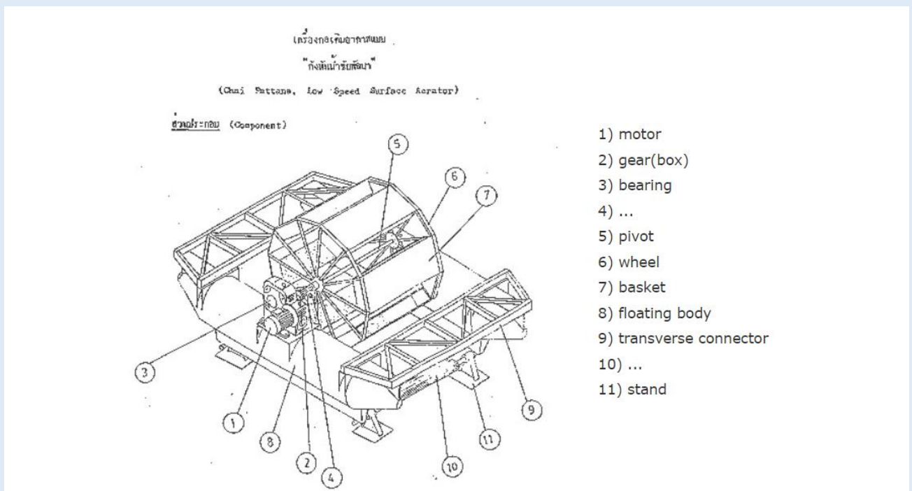
Photo: Drawing of Chaipattana Aerator. (Source: https://www.changpuak.ch )
